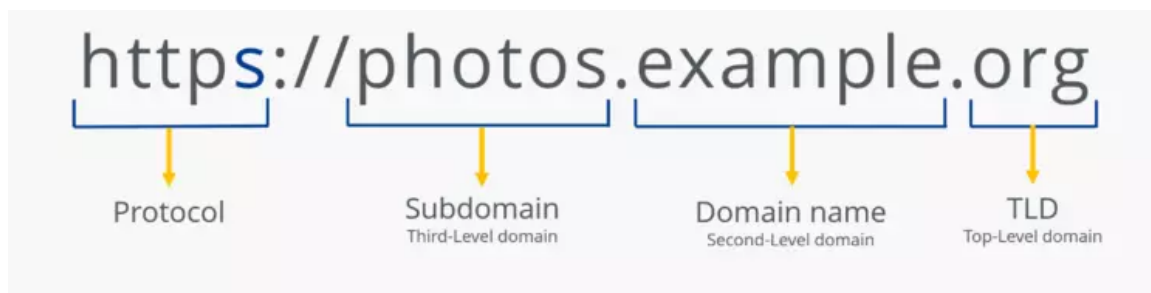
Figure 11.3: Anatomy of a domain
