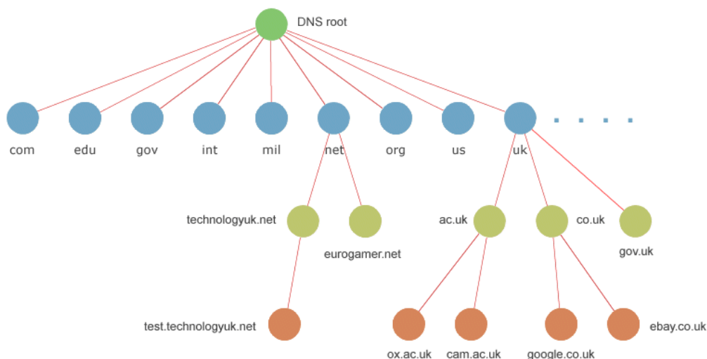
Figure 11.2: DNS Structure
