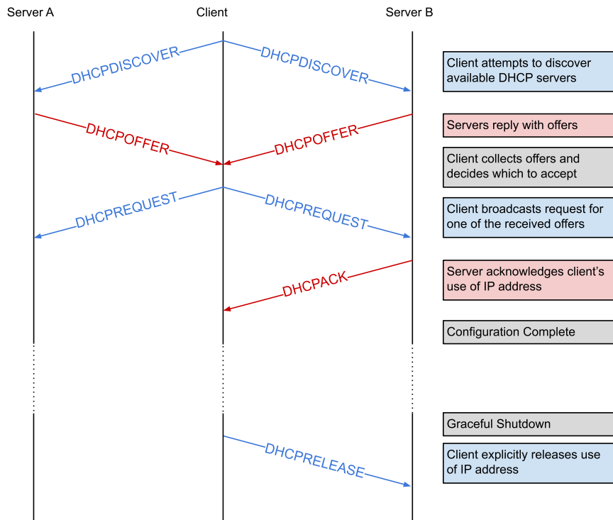
Figure 11.1: DHCP Initial Message Flow
