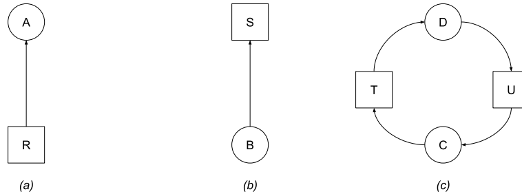
Figure 4.1: Three resource allocation graphs
